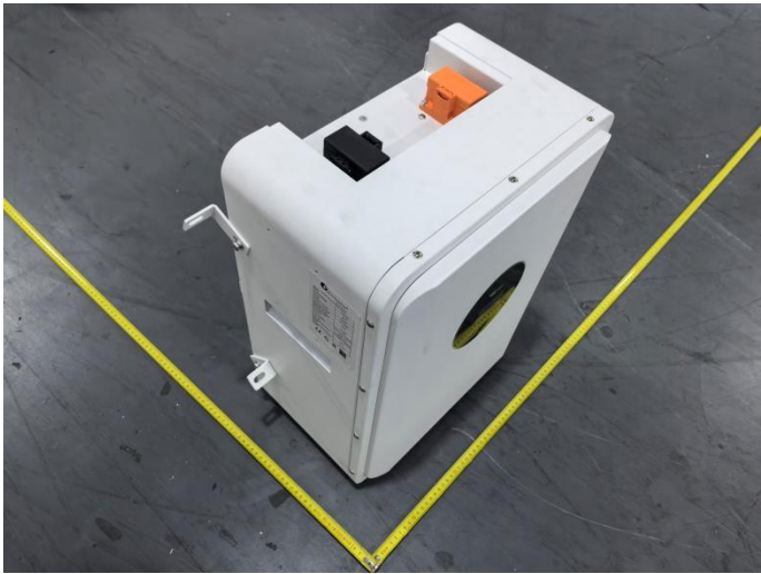
Battery (FLA24250, 25.6V, 250Ah, 6.4kWh)
